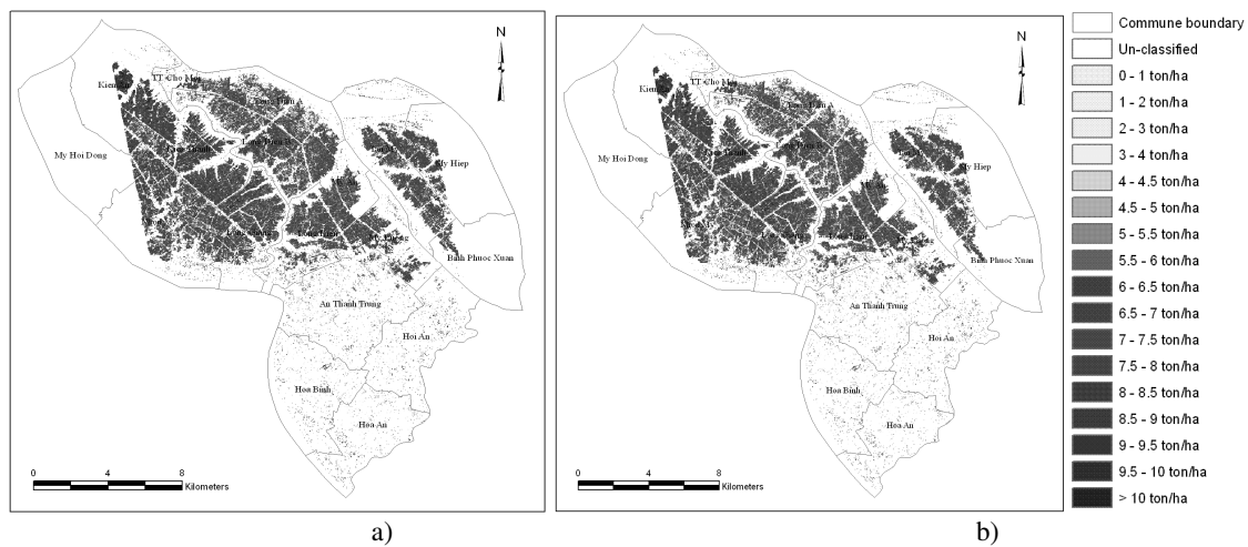
Figure 3. The distribution maps of estimated rice yield in AW 2010 crop at Cho Moi district using five-date (a) and three-date (b) polarisation ratio data.
