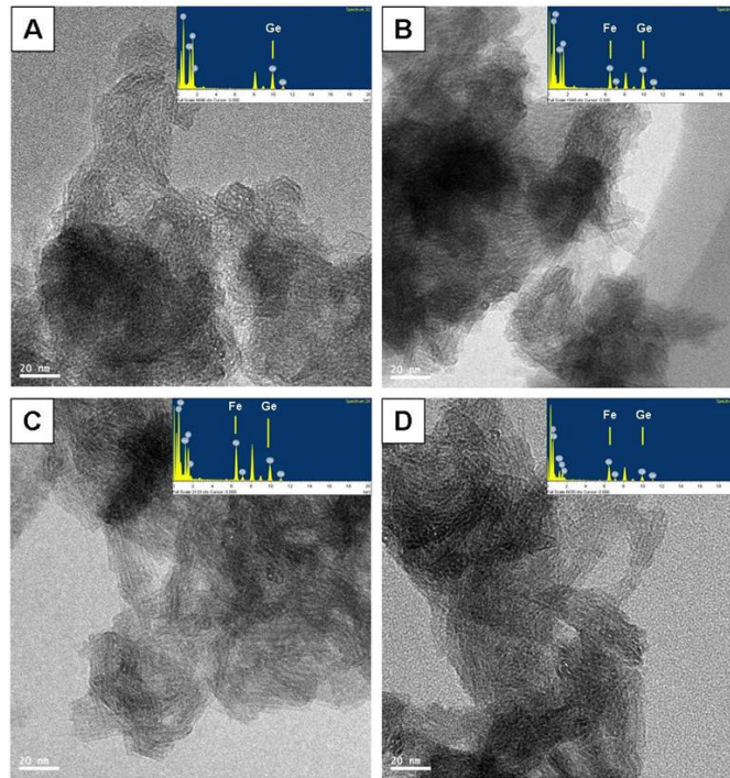
Fig. 4. TEM image of the Fe-substituted aluminogermanate nanotubes synthesized at 2-day aging time and 2 mM initial concentration of aluminum with different Fe/Al ratios of 0 (A), 0.5 (B), 1 (C) and 2 (D).
