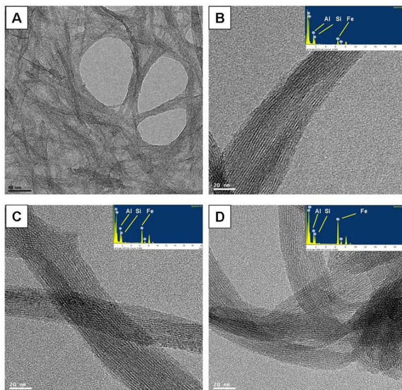
Fig. 3. TEM image of the Fe-substituted aluminosilicate nanotubes synthesized at 2-day aging time and 2 mM initial concentration of aluminum with different Fe/Al ratios of 0 (A), 0.5 (B), 1 (C) and 2 (D).
