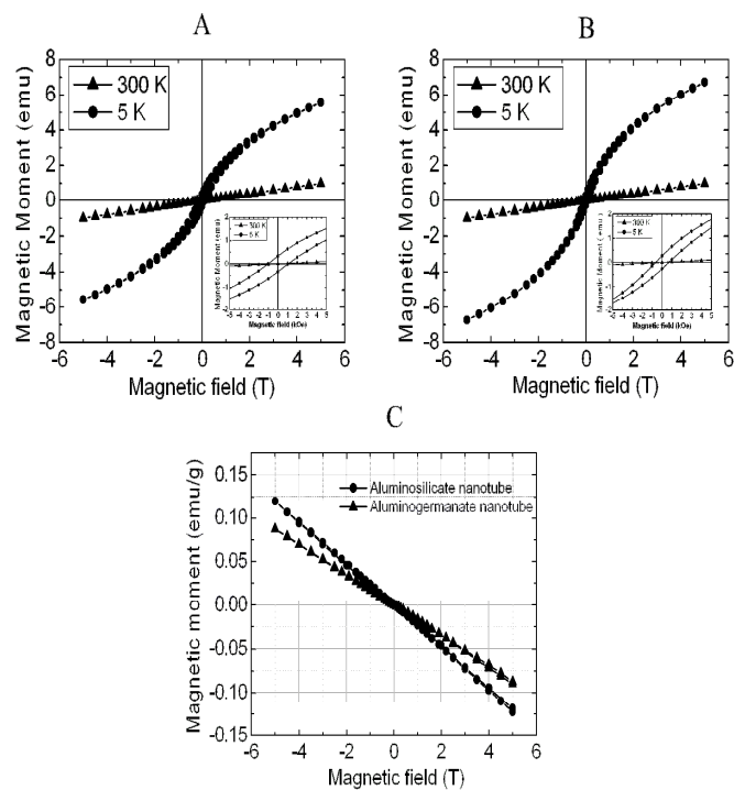
Fig. 5. Hysteresis loops of Fe-substituted aluminosilicate (A) and aluminogermanate (B) nanotubes measured at 300 K and 5 K. Hysteresis loops of aluminosilicate and aluminogermanate nanotubes (C). The insets give better views of the hysteresis loops.
