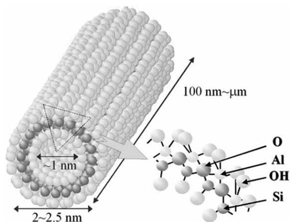
Fig. 1. Structure of imogolite [3]
