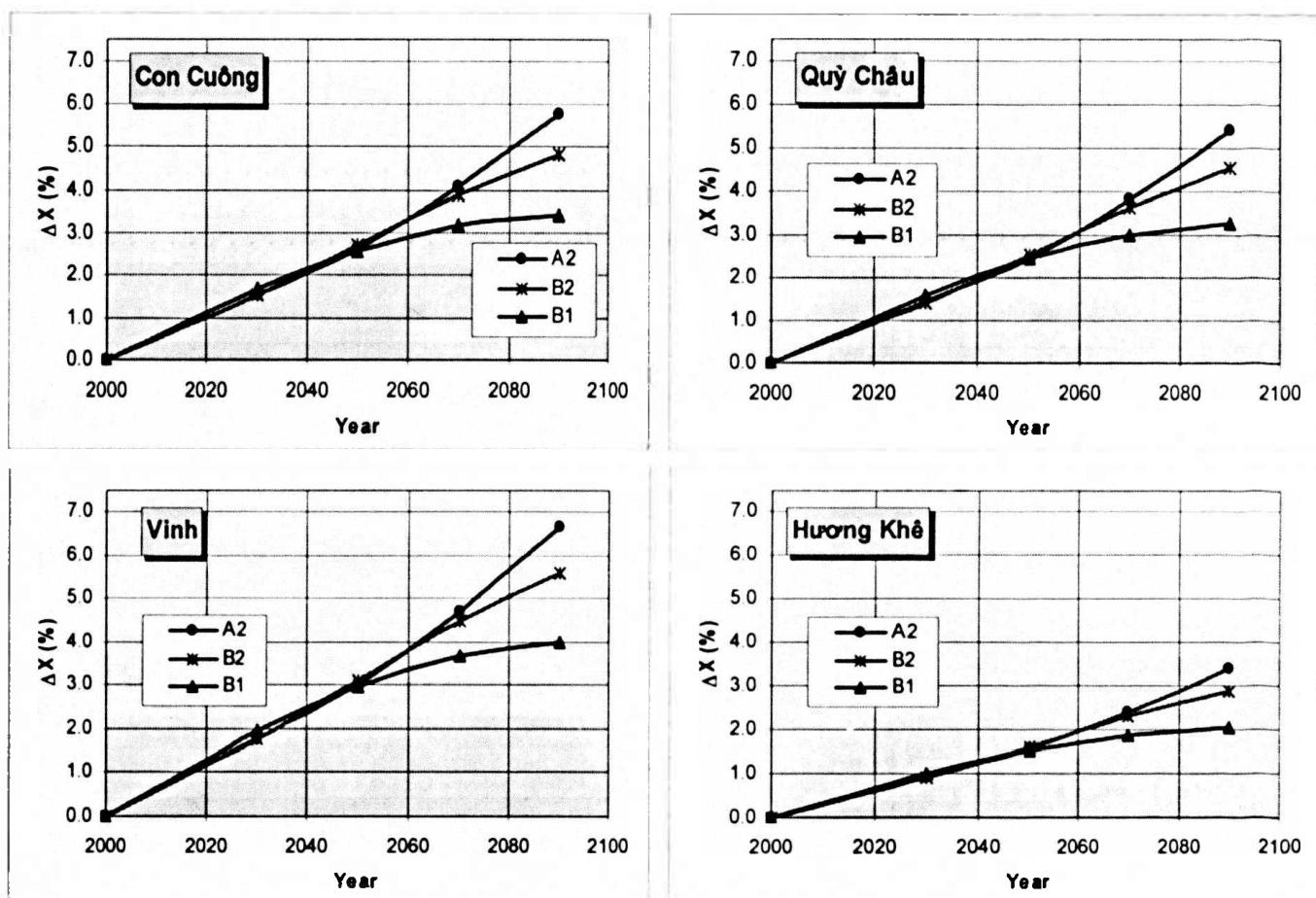
Figure 2. Change in rainfall relative to period 1980-1999 (%) at selected stations in Ca River basin.
