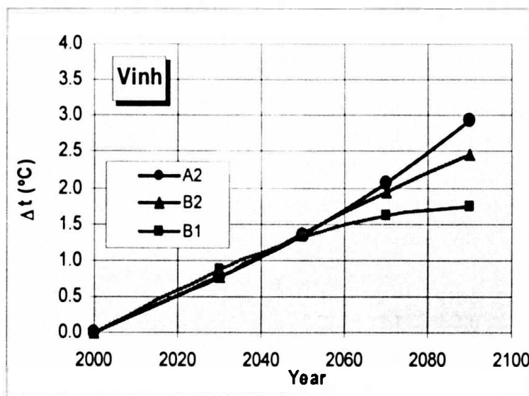
Figure 1a. Changes in annual mean temperature (°C) relative to period 1980-1999 at selected stations.
