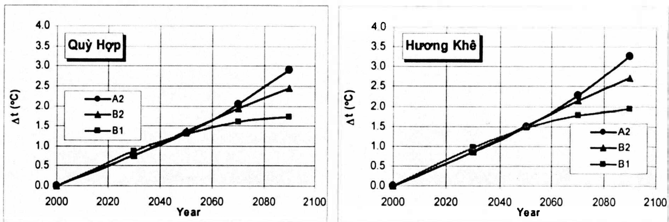
Figure 1b. Changes in annual mean temperature (°C) relative to period 1980-1999 at selected stations.
