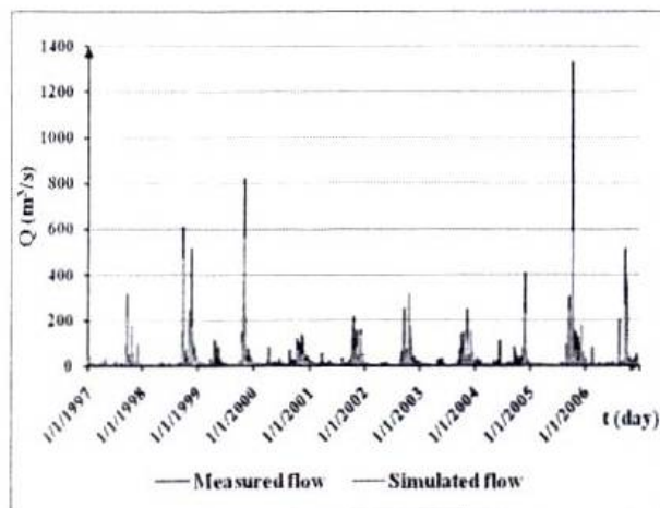
Fig. 2. The time-series comparison of predicted and measured daily streamflow for validation period at Gia Vong station.
