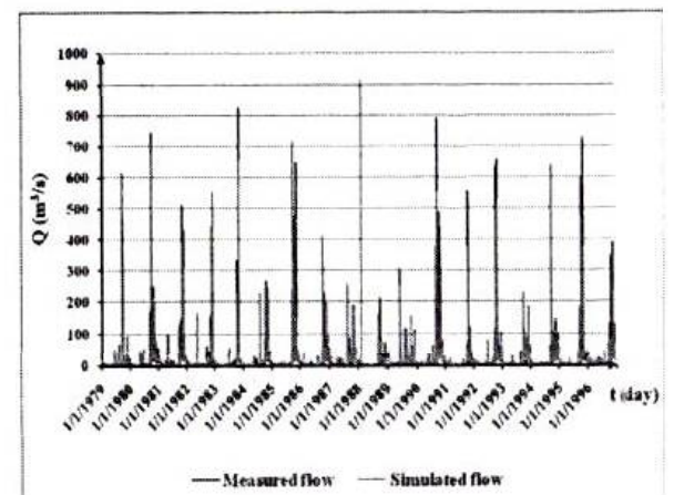
Fig. 1. The time-series comparison of predicted and measured daily streamflow for calibration period at Gia Vong station.
