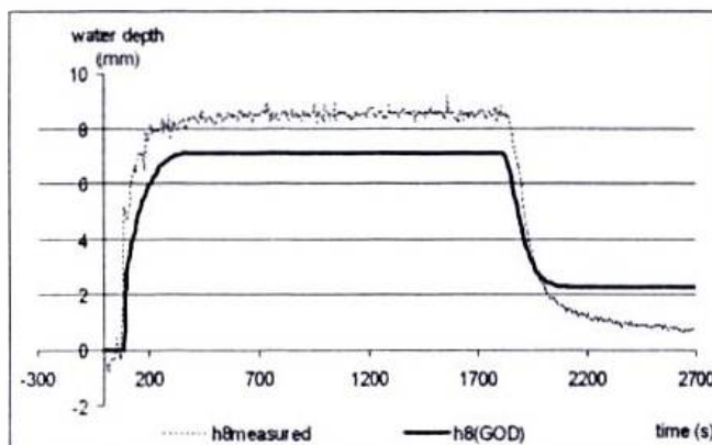
Fig. 11. Comparison of the water depth at point No.8.
