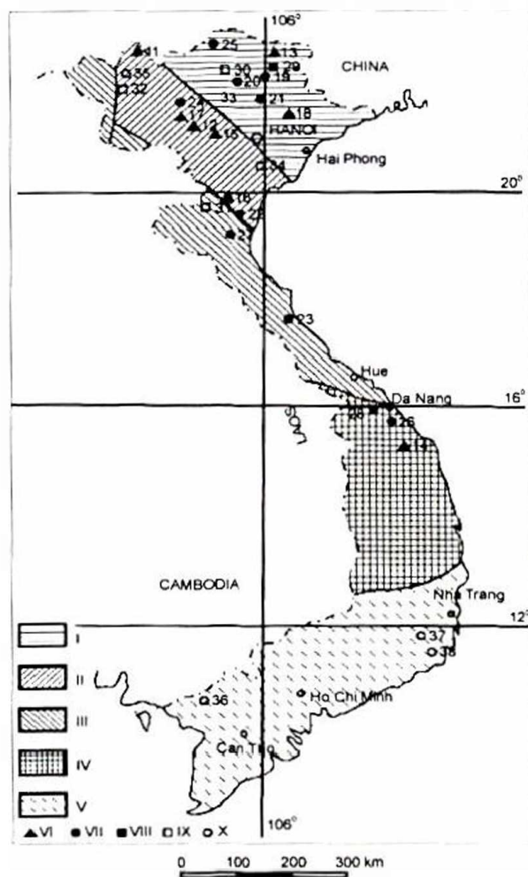
Fig. 3. Sheme of Cu, Pb - Zn, Au, Sb - Hg, Mo ore formations in Vietnam.
