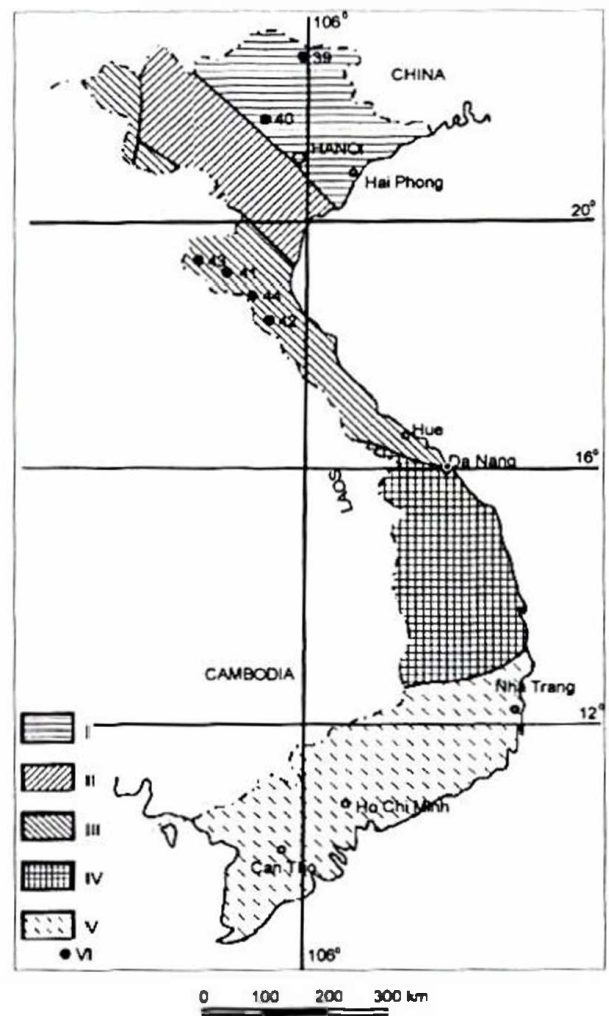
Fig. 2. Sheme of Sn - W ore formations in Vietnam. Metallogenic units: I. Viet Bac; II. Tay Bac; III. Truong Son; IV. Kon Tum; V. Da Lat - Nam Bo; VI. The Sn - W ore deposits (39. Tinh Tuc, 40. Tam Dao, 41. Quy Hop, 42. Kim Cuong, 43. Ban Chieng, 44. Phu Loi).
