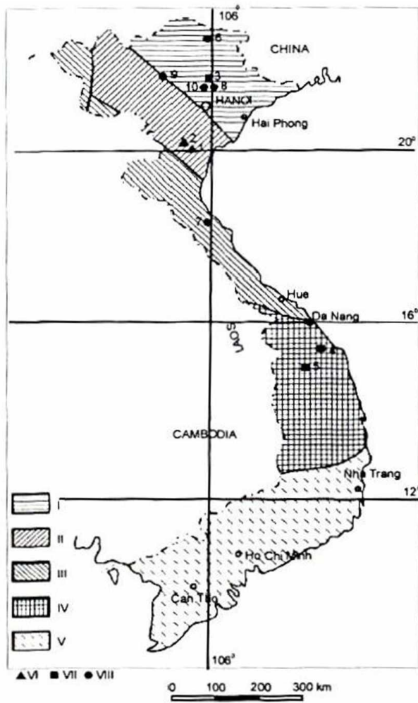
Fig. 1. Sheme of Cr, Ti, Fe ore formations in Vietnam Metallogenic units: I. Viet Bac; II. Tay Bac; III. Truong Son; IV. Kon Tum; V. Da Lat - Nam Bo; VI. The Cr ore deposits (1. Nui Nua, 2. Hon Vang); VII. The Ti ore deposits (3. Nui Chua, 4. Tam ki, 5. Xa Hieu); VIII. The Fe ore deposits (6. Cao Bang, 7. Ha Tinh, 8. Trai Cau, 9. Lang Khuan, 10. Linh Nham).
