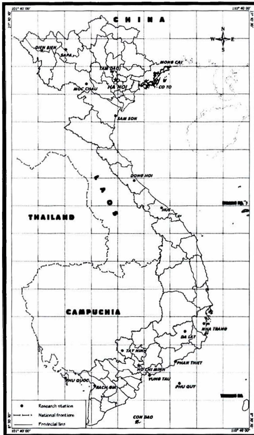
Fig. 1. Distribution of meteorological stations in Vietnam.
