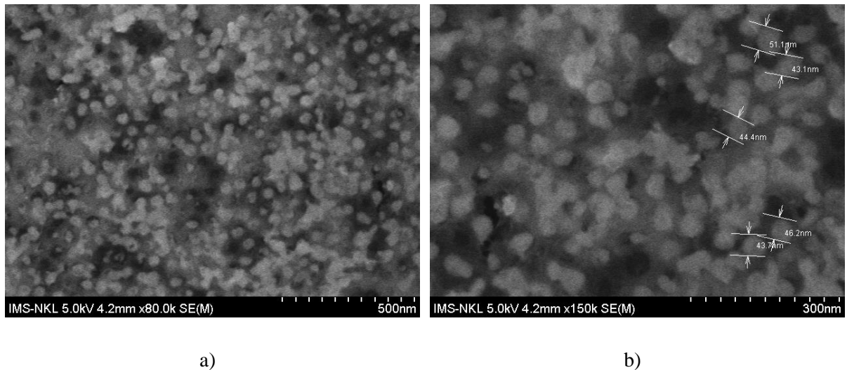
Figure 2. SEM images of the Cu nanodisk 2D array on the AAO template.
