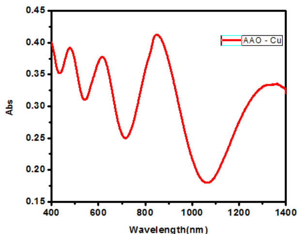
Figure 3: Absorption spectra of the AAO-Cu template
