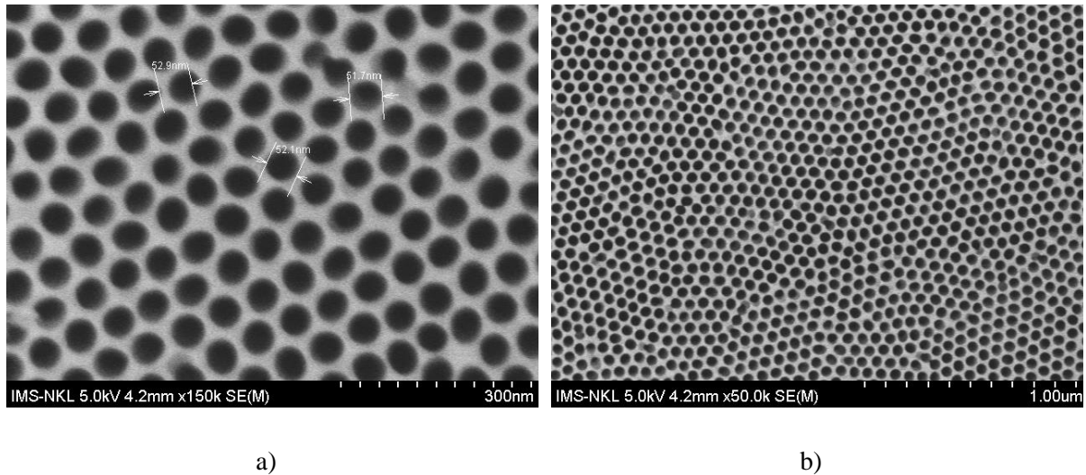
Figure 1. SEM images of the original AAO template showing the diameter of the pores
