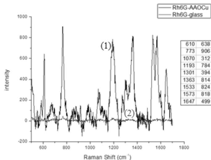
Figure 4. Raman scattering spectra of Rh6G loading on the AAO-Cu template (1) and the Rh6G coated on glass substrate (2).
