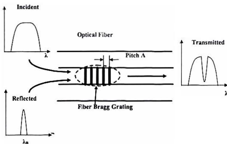
Fig. 1. Structure of the Fiber Bragg Grating.
