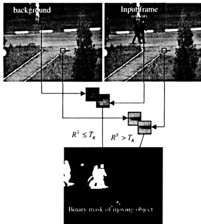
Fig. 5. Schematic diagram for moving object detection.
