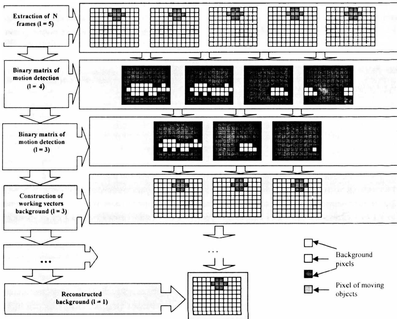
Fig. 1. Schematic diagram for background reconstruction.
