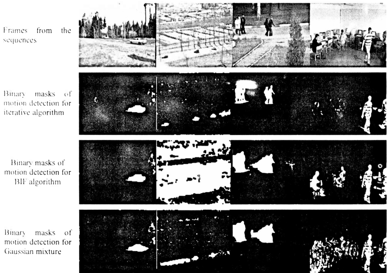
Fig. 4. The motion masks for several sequences.
