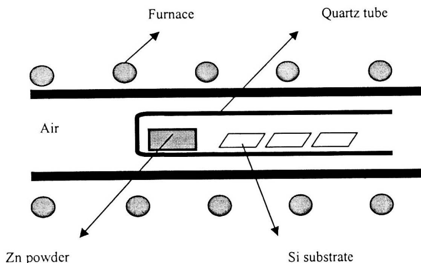
Fig.1. The evaporation system.
