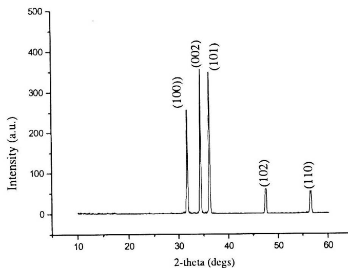
Fig. 2. XRD pattern of ZnO nanotetrapods.
