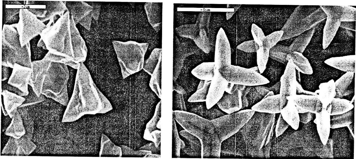
Fig. 3. SEM images of ZnO nano-tetrapods evaporated at (a) 700°C and (b) 800°C.
