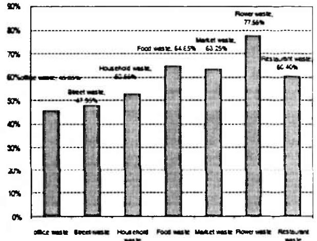
Fig. 3. Organic waste ratio in different waste type, %.
