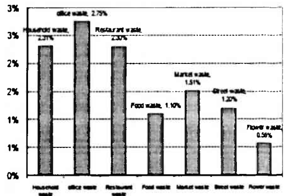
Fig. 4. Metal ratio in each different waste type, %.
