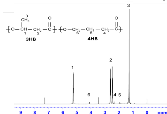
Figure 1. ^1\text{H} NMR spectrum confirming the presence of 4HB monomer in P(3HB-co-4HB) copolymer produced by C. necator H16 using \gamma -butyrolactone as precursor.
