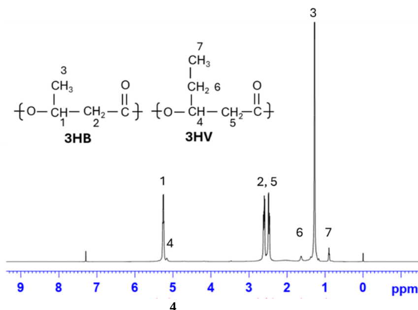
Figure 2. 1 H NMR spectrum confirming the presence of 3HV monomer in P(3HB-co-3HV) copolymer produced by C. necator H16 using sodium propionate as precursor.
